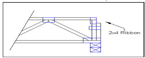
Bottom Chord Bearing
