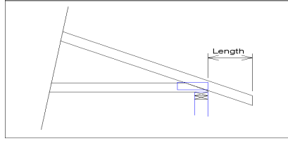
Overhang with plumb cut:
